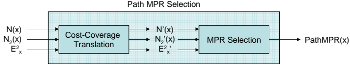
Figure 6. Block diagram for an MPR-based topology selection algorithm. E_x^2 \subset E(G) stands for the set of edges connecting vertices within x \cup N(x) \cup N_2(x) .
