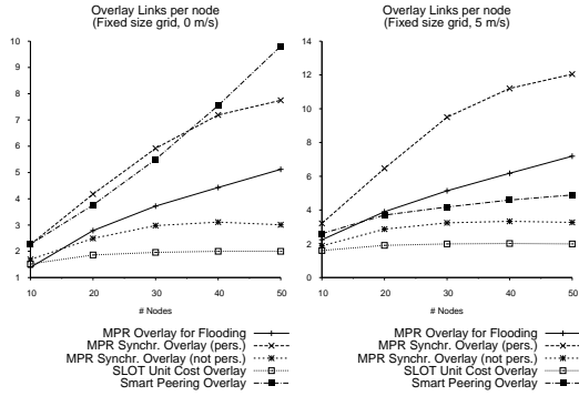
Figure 13. Overlay link density for (a) static scenarios and (b) mobile scenarios (5 m/s).
