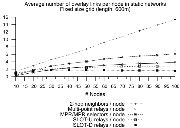
Figure 12. Density of MPR and SLOT overlays in static networks. The SLOT-D simulations are computed with the quantized cost: cost(\bar{x}\bar{y}) = \lceil K \frac{d(\bar{x}\bar{y})}{r} \rceil , with K = 10 and d(\bar{x}\bar{y}) being the Euclidean distance between x and y .
