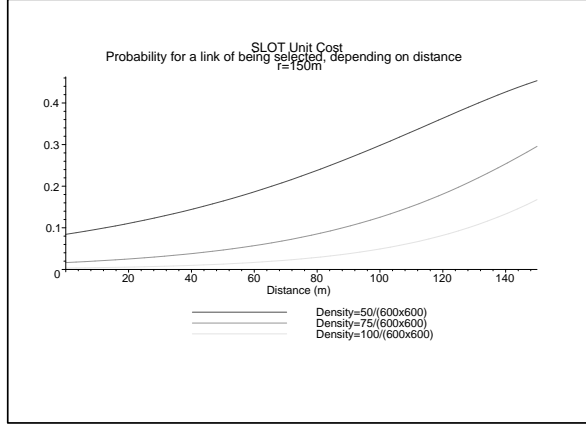
Figure 10. Probability for a link of being selected, under SLOT (unit cost), for different network densities \nu .
