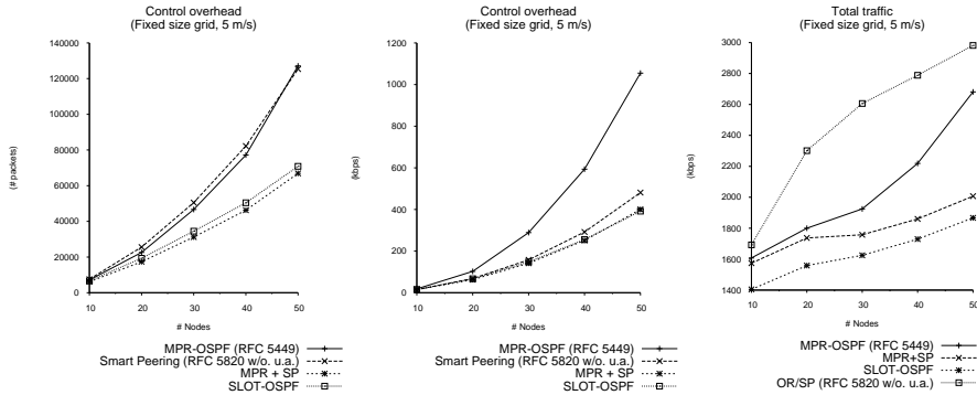
Figure 18. (a) Control traffic overhead, in number of packets, (b) in kbps, and (c) Total (data+control) traffic, in kbps (5m/s).
