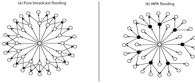
Figure 3. (a) Pure flooding vs. (b) flooding based on the Multi-Point Relays (MPR) principle. Solid dots in (b) represent multi-point relays.
