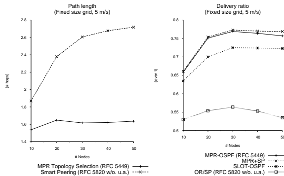
Figure 16. (a) Path length, (b) Data delivery ratio, for 5m/s.
