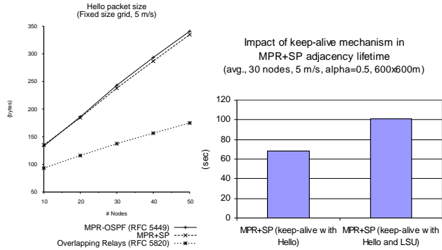
Figure 15. (a) Average size of Hello packets, (b) Impact of keep-alive configuration in adjacency lifetime (fixed grid of length 600m, with speed 5m/s).
