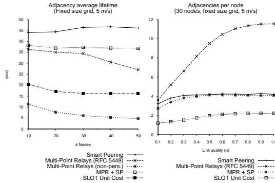
Figure 14. (a) Average adjacency lifetime, depending on the network density, and (b) Average number of adjacencies depending of link quality (30 routers, 5 m/s).
