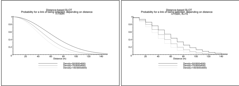
Figure 11. Probability for a link of being selected, under SLOT based on distance, for different network densities \nu .
