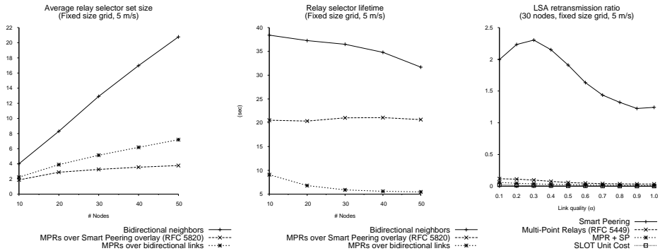
Figure 17. (a) Average size of the MPR set and (b) average relay lifetime (5m/s). (c) LSA retransmission, depending on the link quality (30 routers, 5m/s). The LSA retransmission ratio is the number of backup LSA retransmissions over the number of primary LSA transmissions.
