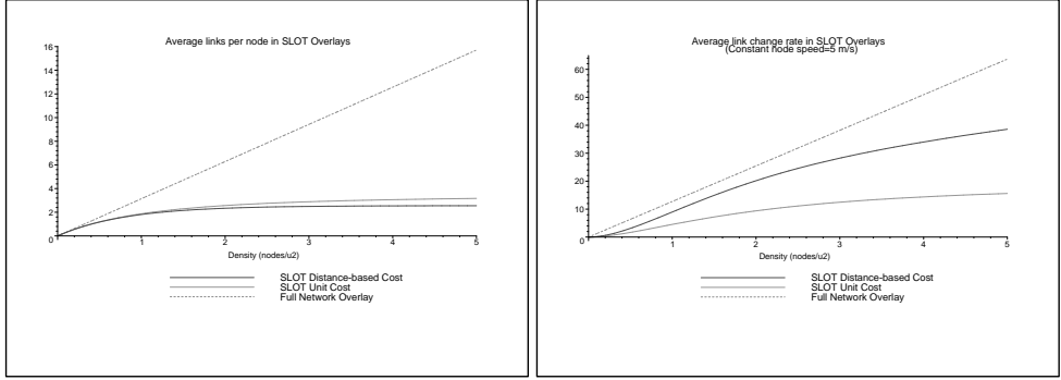
Figure 9. (a) Average SLOT overlay density (links per router), and (b) average SLOT links change, for constant speed s = 5m/s .
