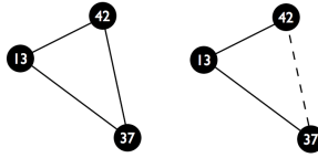
Figure 8. The SLOT triangular elimination under unit link cost. The link connecting routers with the highest ids, 42,37 in the picture, is excluded.
