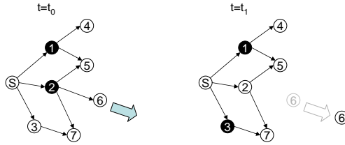
Figure 5. MPR recalculation due to changes in the 2-hop neighborhood. Solid dots represent relays of router S.
