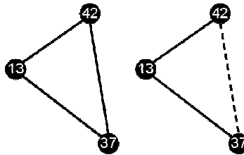
Figure 5. Relative Neighbor Graph (RNG) triangular elimination.
