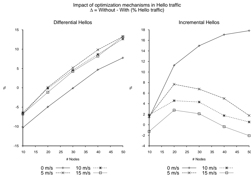
Figure 10. Impact of optimization mechanisms in Hello traffic (%).
