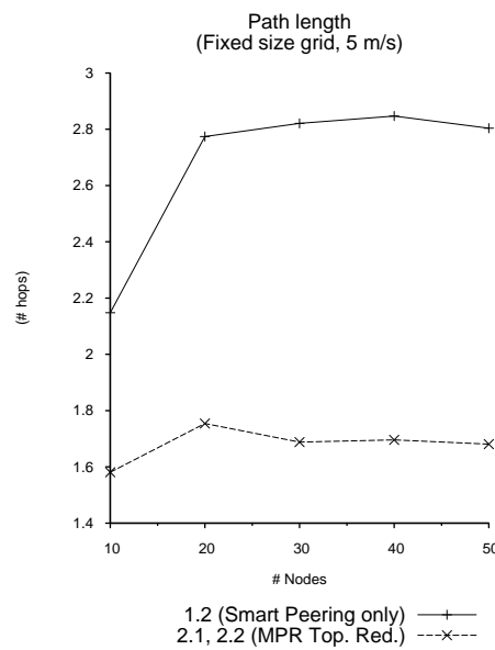
Figure 8. Average path length for data traffic (5 m/s).
