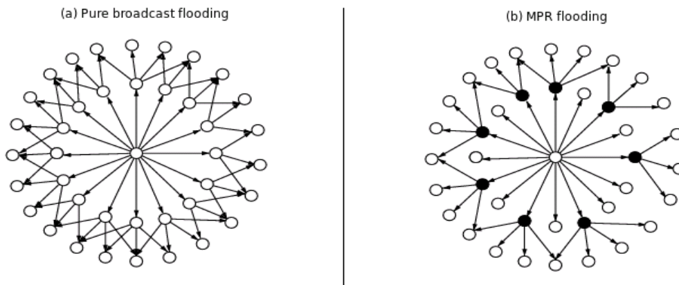
Figure 1. Multi-Point Relays (MPR) flooding vs. pure broadcast flooding.
