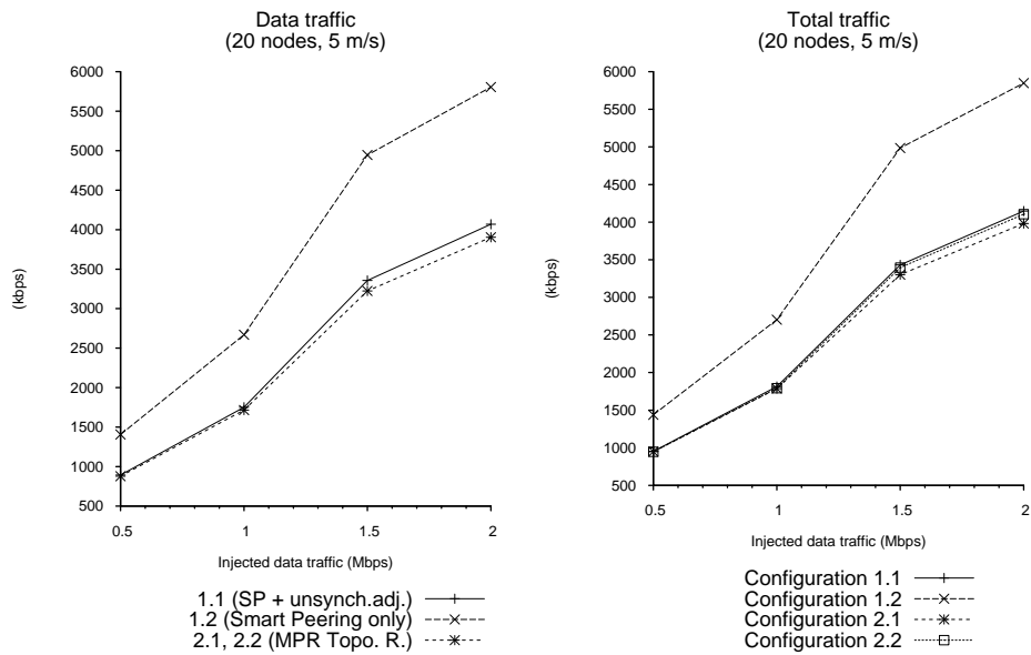
Figure 9. (a) Data traffic and (b) total traffic (data + control) in the network (20 nodes, 5 m/s).
