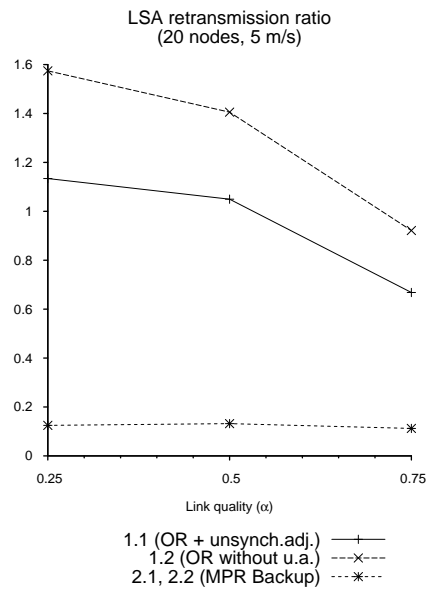
Figure 3. Number of LSA backup retransmissions over number of primary LSA transmissions (LSA retransmission ratio) for configurations 1.1, 1.2, 2.1 and 2.2 (speed: 5 m/s). Details about the simulation environment are in the Appendix.
