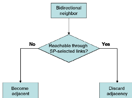
Figure 4. The Smart Peering rule.
