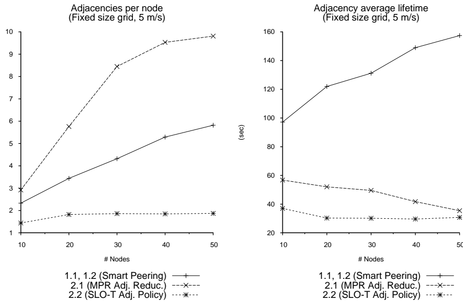
Figure 6. (a) Average number of adjacencies per node and (b) adjacency lifetime in configurations 1.1 and 2 (5 m/s).
