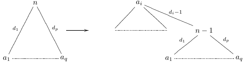
Figure 1: Rewriting rule on agents
