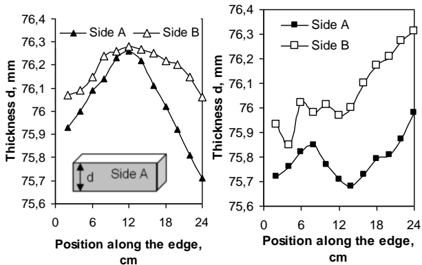
Fig. 5 Typical brick thickness variation for two magnesia-chromite bricks. Sides A and B are opposite each other.
