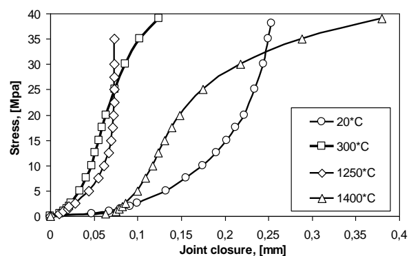
Fig. 4 Joint closure curves of MaC.
