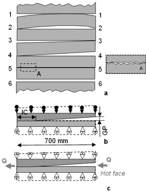
Fig. 2 Possible joint types (a) and FEM model of the joint 4-4 (b, c). The models simulate (b) external displacement loads, (c) own thermal loads.
