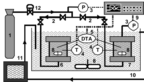
Figure 2 DTA device
