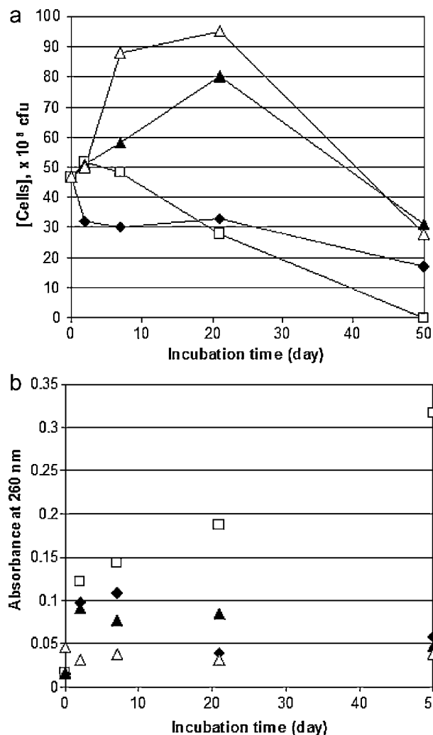
Fig. 3. Evolution of the cell number (a) and nucleic acid content (b) in the supernatant within the 50-day incubation with R. rhodochrous ATCC 29672. Negative control (◆); [C 8 mIm][Tf 2 N] (□); [C 1 COOC 5 mIm][Tf 2 N] (▲) and [C 1 COOC 5 mIm][C 8 SO 4 ] (△).
