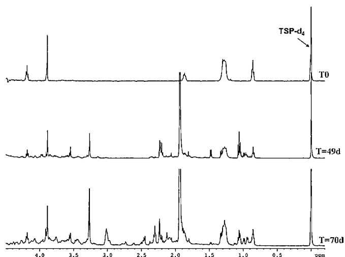
Fig. 2. 1 H NMR spectra (aliphatic region) recorded during the biodegradation of [C 8 mIm][Tf 2 N] by R. rhodochrous ATCC 29672 after T 0 , T 49 and T 70 days of incubation.
