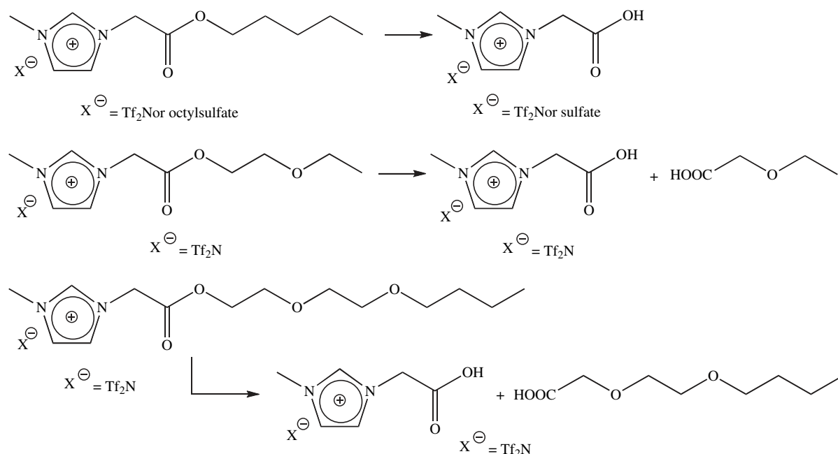
Fig. 4. Metabolic pathways of the studied ILs.
