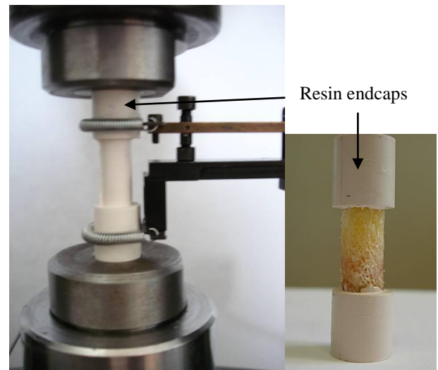
Fig. 2 Experimental device used for compressive tests
