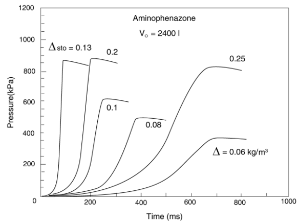
Fig 6 Pressure vs time for different concentrations.
