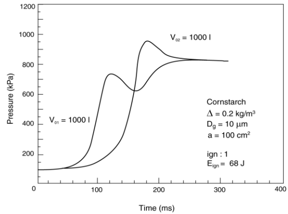
Fig 8 Pressure vs time in both compartments.
