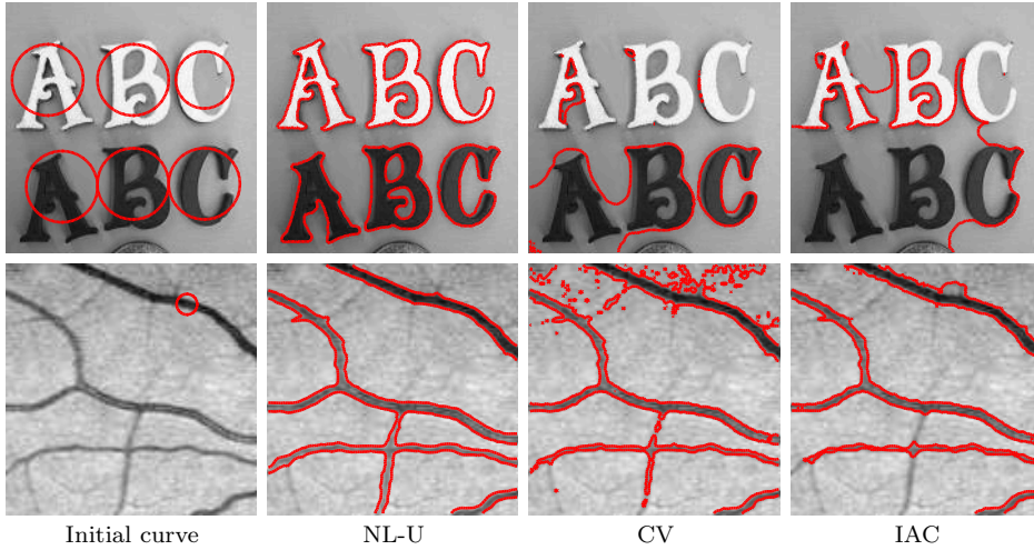
Fig. 5.4: Grayscale images segmentation. Final curves of our un-normalized model NL-U, CV and IAC.
