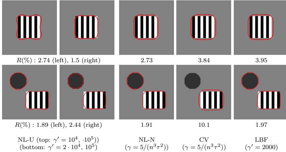
Fig. 7.1: Comparison of models with the Wasserstein distance function (7.2). R(\%) indicates the mis-matching rate between a resulting curve and the ideal curve exactly located on the object boundary.
