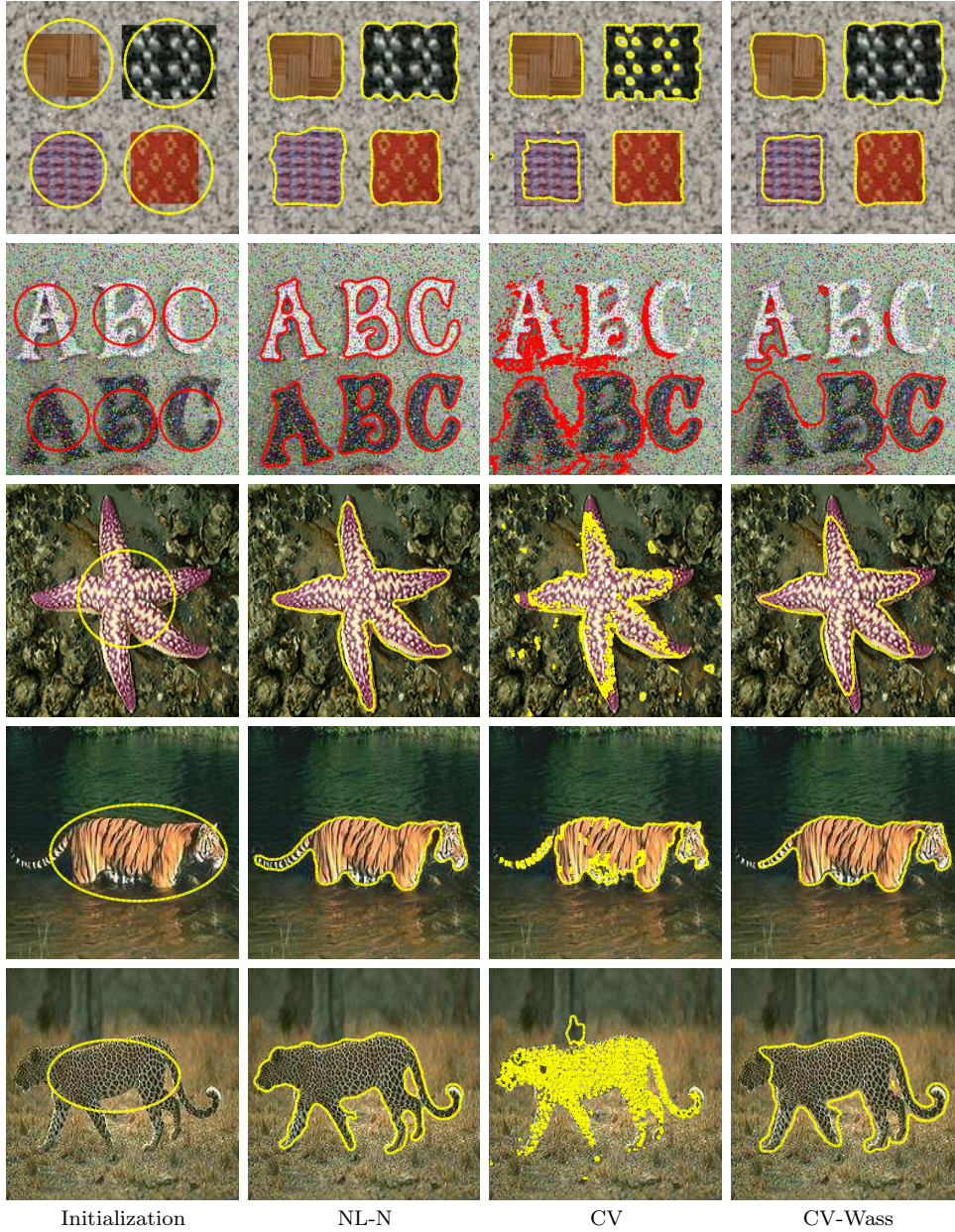
Fig. 7.4: Texture segmentation of our NL-N model (3.5) with the sliced Wasserstein distance (7.3) with |\Theta| = 3 fixed directions, and comparison with the vector-valued Chan-Vese (CV) model [12] and the extended work (CV-Wass) [2] of [40].
