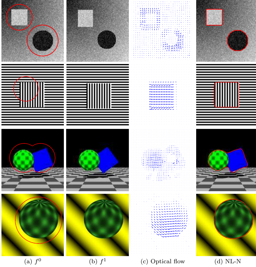
Fig. 8.2: Segmentation of moving objects with our NL-N model (3.5) and the motion distance (8.1).
