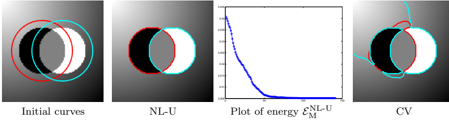
Fig. 9.2: Segmentation results of multi-phase method MI with the NL-U energy and the CV energy.
