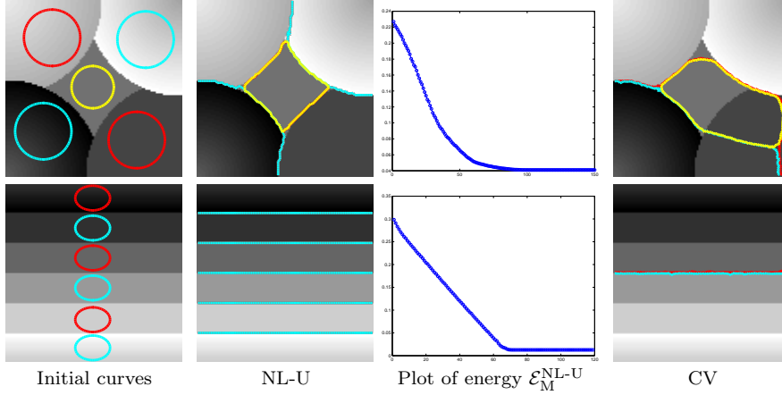
Fig. 9.1: Segmentation results of multi-phase method MR with the NL-U energy and the CV energy.
