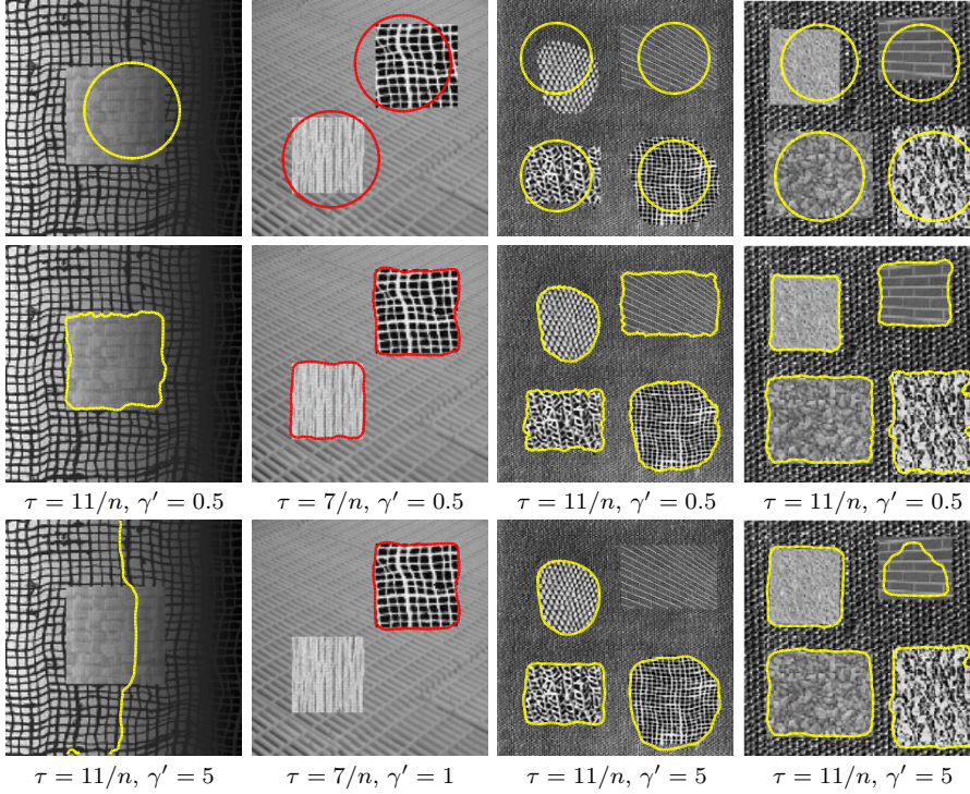
Fig. 7.3: Segmentation results with Wasserstein distance (7.2). Top row: Initial curves. Middle: Results of our NL-N model (3.5). Bottom: Results of the CV model extended with Wasserstein distance.
