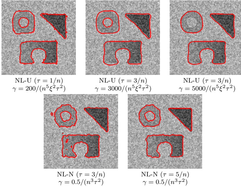
Fig. 5.6: Comparison of our un-normalized (3.2) and normalized (3.5) models using the L^2 distance (5.1).
