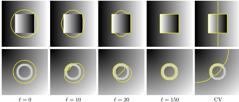
Fig. 5.1: Curve evolution for the segmentation of two images with spatially varying background and object using NL-U, and comparison with CV. \ell is the iteration number.
