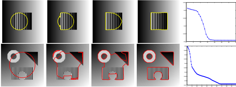
Fig. 7.2: Segmentation results with Wasserstein distance (7.2). Left: Curve evolution using our NL-N model (3.5). Right: Plot of energy \mathcal{E}(\varphi^{(\ell)}) vs iteration \ell .
