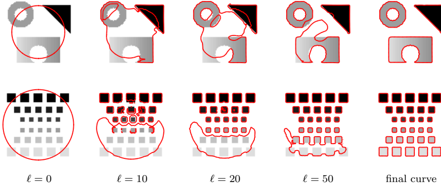
Fig. 5.2: Curve evolution for the detection of objects with spatially varying object, or with several separated objects with different intensities, using NL-U model. \ell is the iteration number.
