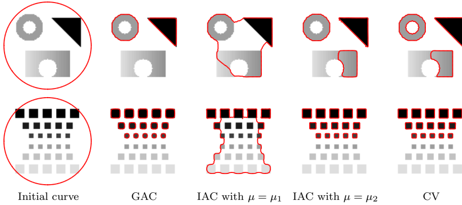
Fig. 5.3: Comparison of CV, GAC and IAC (different \mu values).
