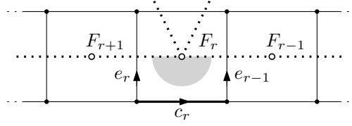
FIGURE 24. By construction of the sequence F_1, \dots, F_{n+1} , the grey sector does not contain any edge of the dual spanning tree \widehat{T} . Hence, the path c_r stays in the spanning tree T .
