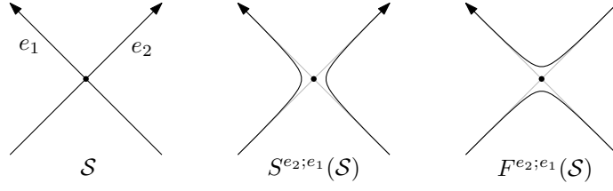
FIGURE 21. The operations S^{e_2;e_1} and F^{e_2;e_1} can be understood as acting locally at the common origin of e_1 and e_2 . From this point of view, the fact that e_1 and e_2 are on the same loop or not does not matter. The only difference is, in the case of the operation F^{e_2;e_1} , the direction in which the lower strand is traversed. In fact, in this case, the orientation of the loop \tilde{l} itself is arbitrary. We chose to let it traverse e_1 positively, but the other choice would not make any difference, since this operation is used only in the real and quaternionic cases, where a Wilson loop is not altered by changing the loop into its inverse.
