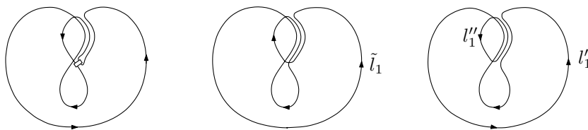
FIGURE 20. The left-hand side of this picture shows how (103) applies in the present context. The white box represents, as on Figure 16, the Casimir operator of \mathfrak{u}(N, \mathbb{K}) . The two other pictures show the loops which arise in \partial_{t_3} \mathbb{E}_t [W_l] . Note that the edge e_4 is traversed more than once by these loops.
