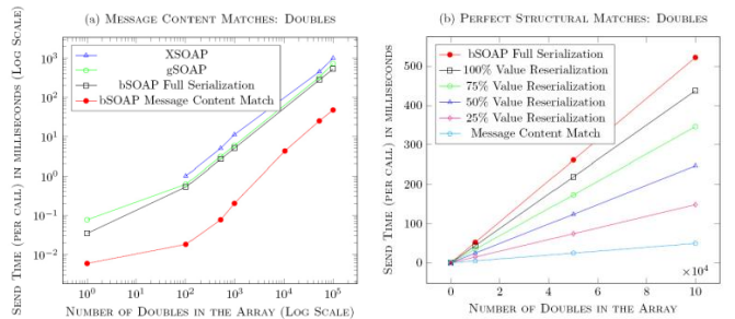
a. Comparing bSOAP, to alternative approaches, i.e., gSOAP [77] and XSOAP [63]. b. Serialization time, when various percent-tages of stored values are re-serialized.
