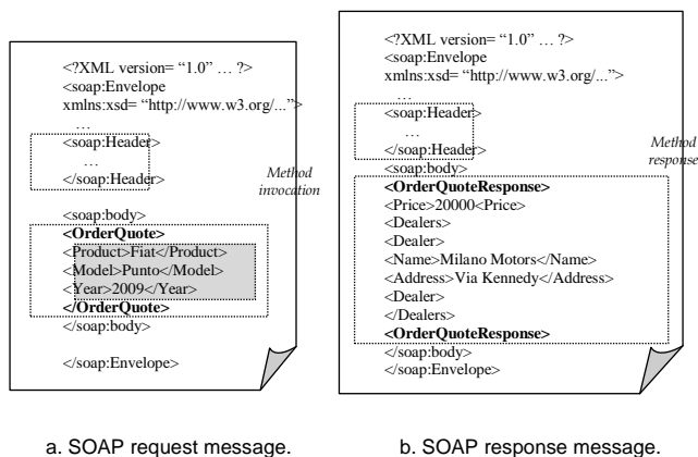
Fig. 2. Sample SOAP request and response messages.
