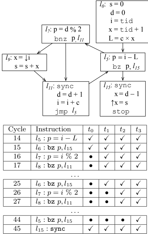
Figure 2: (Top) A \mu -SIMD program. (Bottom) An execution trace of the program. If a thread t executes an instruction at cycle j , we mark the entry (t, j) with the symbol \checkmark . Otherwise, we mark it with \bullet .
