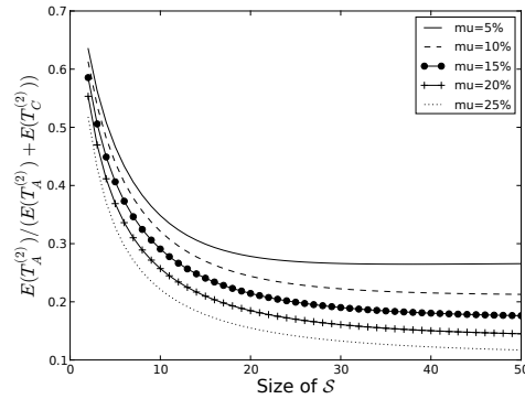
(b) E(T_A^{(2)}) / (E(T_A^{(2)}) + E(T_C^{(2)})) as a function of the size s of \mathcal{S} . We have \alpha = \beta , and c = 10 .
