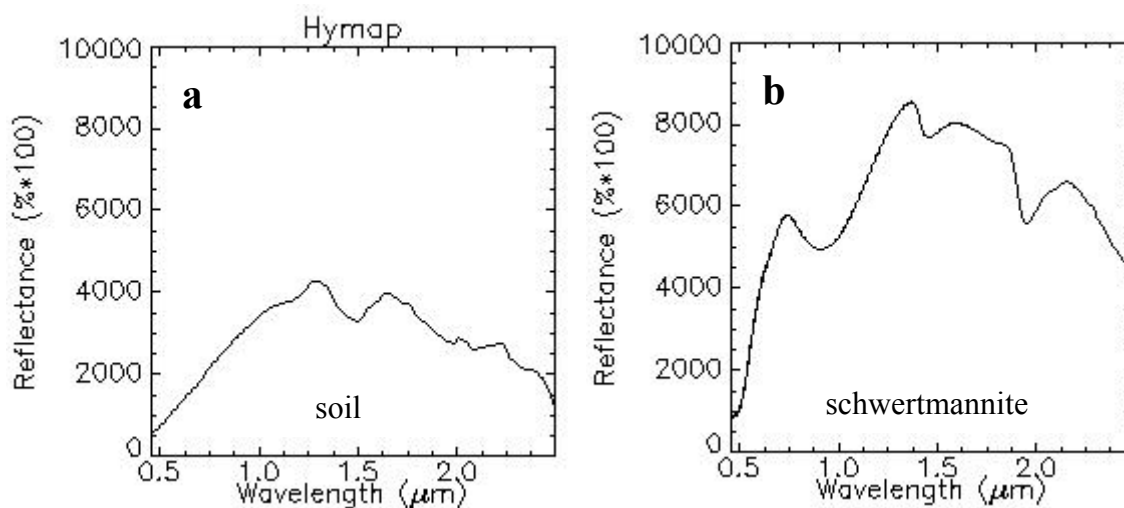
Figure 4. (a) Spectra from soil over the host rock extracted from Hymap data (b) Spectra from schwertmannite \text{Fe}^{3+}_6\text{O}_{16}(\text{OH})_{12}(\text{SO}_4)_2 resampled to Hymap data [7].
