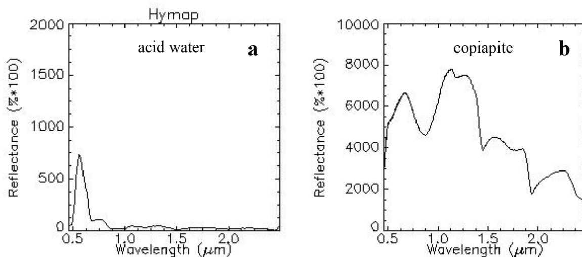
Figure 3. (a) Spectra from acid water extracted from Hymap data (b) Spectra from copiapite ( \text{Fe}^{2+}\text{Fe}^{3+}_4(\text{SO}_4)_6(\text{OH})_2 \cdot 20(\text{H}_2\text{O}) ) resampled to Hymap data [7].
