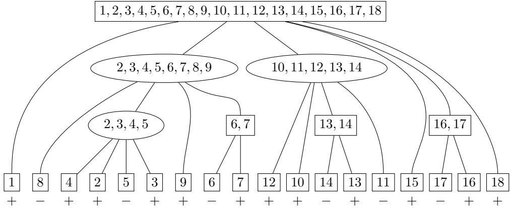
Figure 1: The strong interval tree \mathbf{T}([1 \bar{8} 4 2 \bar{5} 3 9 \bar{6} 7 12 10 \bar{14} 13 \bar{11} 15 \bar{17} 16 18]) . Vertices are labeled by the strong intervals. There are three non-trivial linear vertices (rectangular) and three prime vertices (round). The root and the vertex \{6, 7\} are increasing linear vertices, while the linear vertices \{16, 17\} and \{13, 14\} are decreasing.
