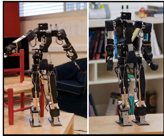
Fig. 1. The Acroban platform: a bio-inspired and compliant humanoid robot (more informations and videos on our website: http://flowers.inria.fr/acroban.php )
