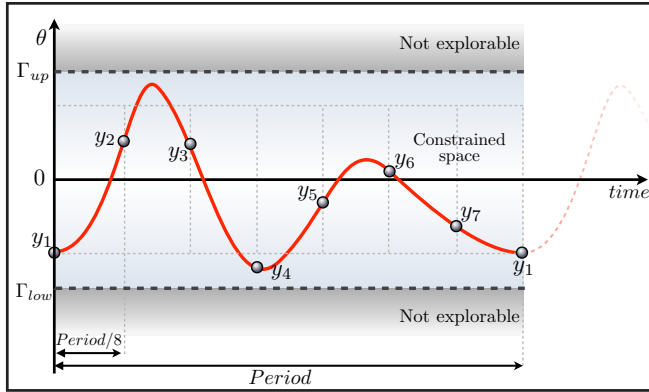
Fig. 4. CPGs are generated by key-points set in the joint position space. This space is constrained (see IV-A2). A bezier curve defined by these key-points generates the motor commands over time.
