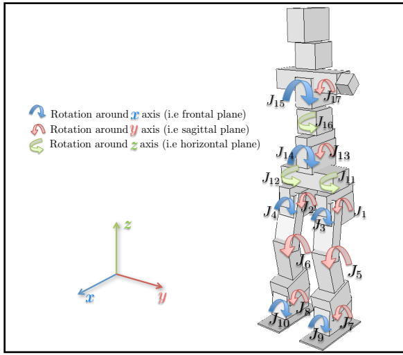
Fig. 3. Overview of actuated joints in our experiments. Names of DoF refer to the order of releasing during learning
