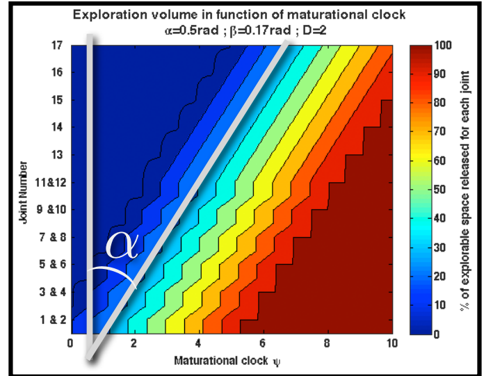
Fig. 5. Releasing way for each degrees of freedom in function of the three parameters ( \alpha , \beta and D ) and the maturational clock \psi . With these parameters, at \psi = 0 , joints 1 & 2 have around 10% of their motor space available. All others joints can not move.
