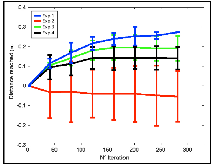
Fig. 7. Learning curves for each experimental parameters. The y-axis represents the distance traveled by the robot and the x-axis the iteration number. The best curve is the blue one with strong maturation constraints. With these parameters, the robot was able to travel around 30cm in 9sec. The best result is close to the velocity of the real robot working with a hand-tuned controller
