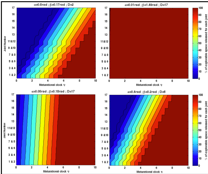
Fig. 6. Figure showing the four parameters sets chosen to compare the learning efficiency in function of the way to release maturational constraints
