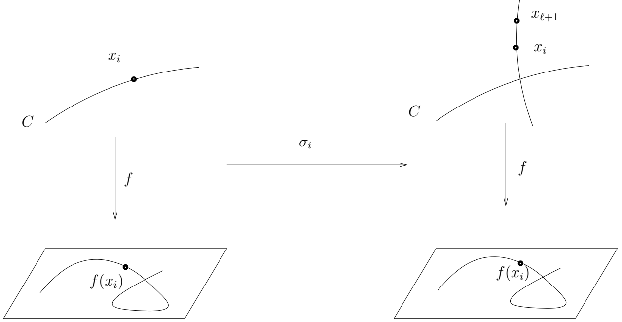
FIGURE 2. L'application \sigma_i .
