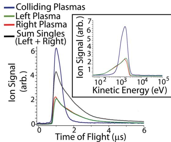
Figure 2. (Main) Ion TOF signals for colliding plasmas (dark blue trace) and single seed plasmas (red and green traces). The Faraday cup was positioned normal to the target. (Insert) TOF signals converted to kinetic energy distributions for single ‘seed’ plumes and colliding plasmas system.
