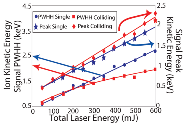
Figure 5. The variation of the Profile Width at Half Height (PWHH) and peak position of the ion energy distribution normal to the target with incident laser energy for colliding plumes. The arrows point to the relevant axes for each trace. In the case of the single plasma plume the total energy into the focal spot on the target was 100% of the value shown on the horizontal axis. In the colliding plasma case the total energy in each of the seed plasmas was 50% of the values shown.
