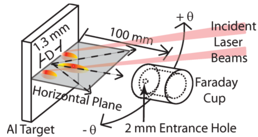
Figure 1. Schematic diagram of the experimental configuration (not to scale). The seed plasmas were separated by a distance of 1.3 mm, the Faraday cup was located at a distance of 100 mm from the target and the entrance aperture of the Faraday cup was 2 mm in diameter.
