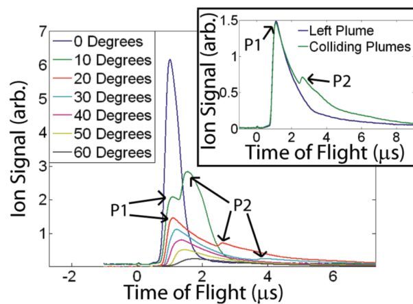
Figure 4. Main: Angle-resolved TOF signal for colliding plasmas for a range of angles of detection (main). Insert: Comparison of the colliding plasma TOF signal with that of a single plasma plume at a detection angle of 20°.
