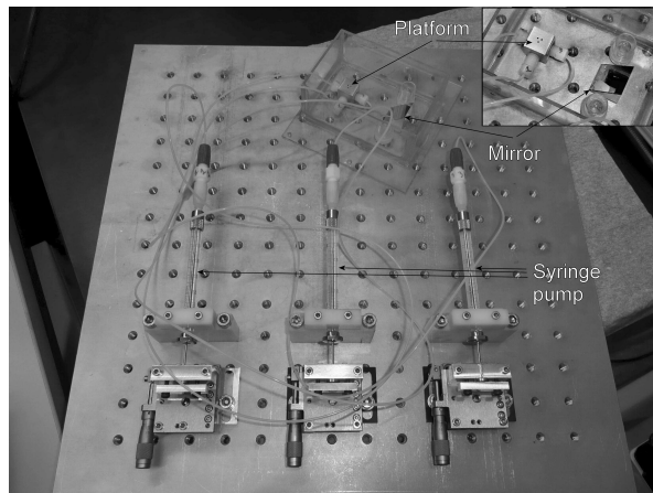
Fig. 13. View of an enhanced version of the test bed. The picture shows the manual micropositioning stages used as syringe pumps, and the test cell where the platform is immersed in a liquid. The illustrated version uses PTFE hoses and gas tight syringes
