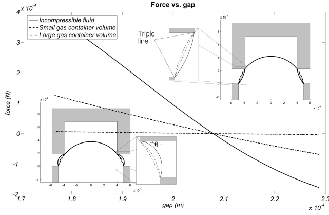
Fig. 6. Illustration of force vs. gap evolution for different gas system volume ( s_{\text{bottom}} = 10^{-3} m, s_{\text{top}} = 0.8 \cdot 10^{-3} m, \gamma = 72 \cdot 10^{-3} Nm ^{-1} , h_{\text{init}} = 0.4 \cdot 10^{-3} m and P_0 = 101325 Pa). If the gas container is large (here 10^{-6} m ^3 ), a small variation of volume will not change pressure significantly, so the pressure variation and bubble curvature variations are small. The stiffness of the bubble is in this case small. On the contrary, if the gas system volume is small (here 10^{-8} m ^3 ), any volume variation will induce a significant change in the gas pressure, and the shape of the bubble will vary significantly. The stiffness of the bubble is therefore larger. We have also indicated the case of an incompressible fluid, for which the stiffness is even larger. Both illustrations show the shape of the interface for the minimal (left) gap and maximal (right) gap
