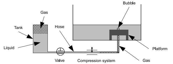
Fig. 3. Illustration of volume controlled bubble generator for the prototype. A bubble is grown by squeezing the flexible hose joining the platform and a container
