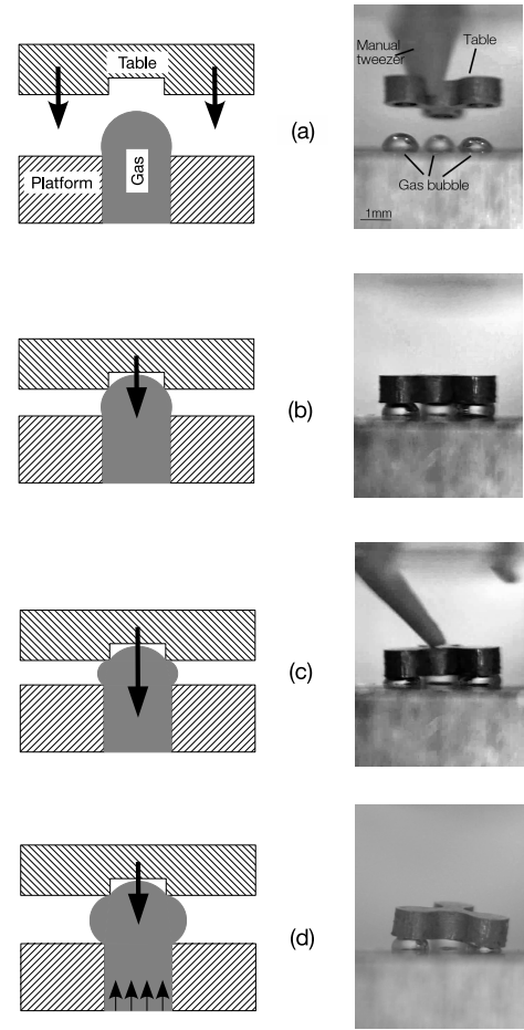
Fig. 7. Illustration of the capillary driven robotic table concept. Three bubbles are generated from the platform, and the table is dropped on the bubbles. The table is automatically self centered above the platform (a). To counterbalance the force exerted by the table, the bubbles change their shape as the gap distance reduces (b). If supplementary force is applied, the table moves down as the bubble generated force increases (c). It is also possible to lift or tilt the table by injecting more gas in the bubbles (d)
