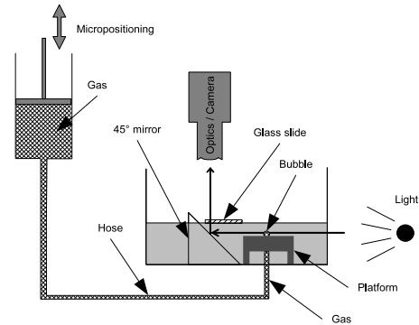
Fig. 12. Illustration of volume controlled bubble generator for the prototype. Three bubbles are grown by injecting gas from syringes actuated by a micropositioning stage. The table is then deposited on the bubbles
