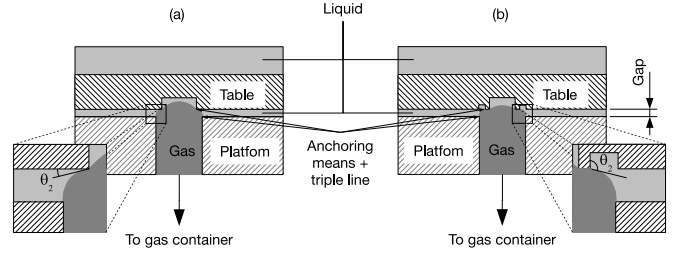
Fig. 2. Illustration of one leg of the table. A bubble is generated from the platform and lift the table. The anchoring means are in this case geometrical changes that improves the fixation of the line where solid-liquid and gas touches each other (triple line)
