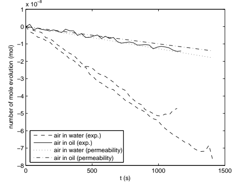
Fig. 11. Comparison of permeability model of gas permeation through flexible hoses with experiments. When the liquid is silicone oil, the permeability of the silicone hoses explains the origin of gas mole decrease in the system. When the liquid is water, only a part of the gas mole decrease is explained by the permeability of the silicone hose, the difference is probably due to gas dissolution in the water
