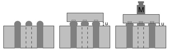
Fig. 5. Principle of the experimental validation of bubble stiffness model. First a single bubble is generated from each hole of the platform. Then the table is layed on the bubbles and the distance u between the table and the platform is measured. Finally, different known masses are added successively and the evolution of u is measured
