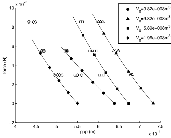
Fig. 9. Experimental validation of the vertical force model. The unfilled symbols represent the measurements, the filled symbols on curves represent the solution from the model corresponding to the experimental setup conditions
