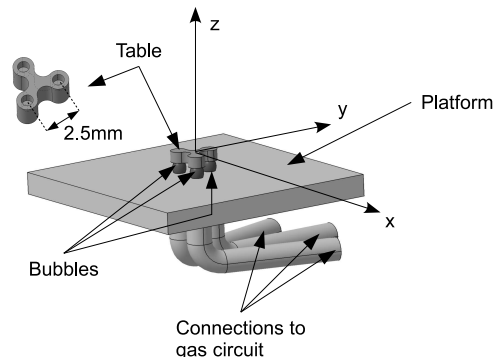
Fig. 1. Schematic view of the device, composed of a compliant table lying on 3 bubbles generated from a platform
