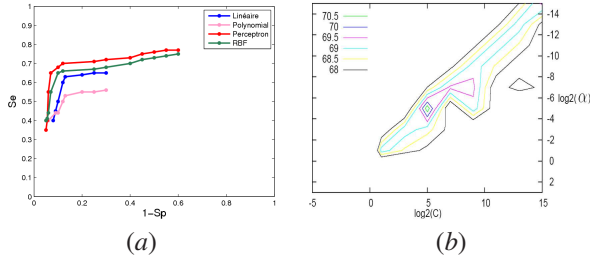
Figure 2: Classifier design: (a) ROC curve obtained by 4 different kernels (b) hyper-parameters setting of C-SVM classifier with RBF kernel. The training set is obtained by combining MCD-DCD with GLCM descriptors.
