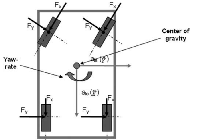
Fig. 6. Single-lane one-wheel model.
