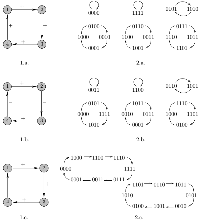
Fig. 1. Figures 1.a., b. and c. represent three different Boolean automata circuits of size n = 4 . That of figures 1.a. and b. are positive while that of figure 1.c. is negative. Figures 2.a., b. and c. picture the iteration graph of these networks, that is, the graph that represents their dynamics. The nodes of these graphs are the elements of \{0, 1\}^n and an arc (x,y) exists in this graph if and only if F(x) = y . Every strongly connected component of the iteration graph corresponds to an attractor of size the number of elements in this component. Note that in all three cases here, all elements belong to an attractor. This is usually not the case with arbitrary Boolean automata networks which are not circuits.
