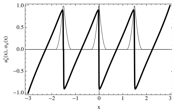
(b) At the end of the loading phase three transverse cracks are obtained, represented by the localization field \alpha on a narrow zone. In our regularized formulation, discontinuities of the displacement are replaced with zones with very high gradient.
