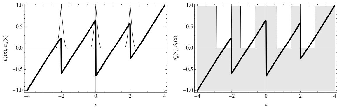
(b) Plot of the displacement and damage fields, the film exhibits three transverse cracks at the end of the loading phase.
