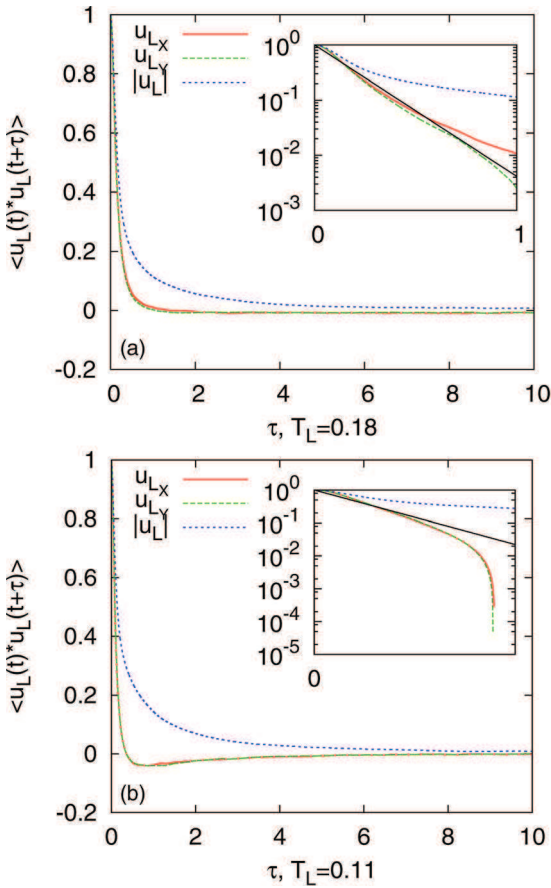
FIG. 9. (Color online) Lagrangian velocity autocorrelation for periodic and circular geometry. a and b correspond to the periodic and circular domains, respectively.
