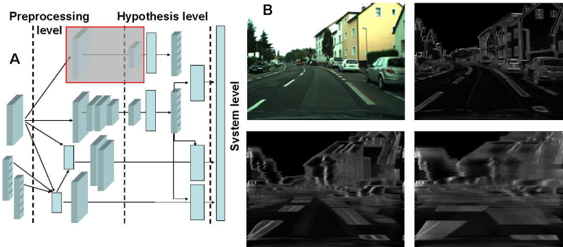
Fig. 4 Performance example of symmetry-based object detection. A) Embedding into processing system. B) Input image and generated multi-scale confidence map. A total of K = 8 scales is used for symmetry, corresponding to filters of pixel height h = 3 and half-width \frac{h}{2} = 5, 9, 13, 18, 25, 35, 49, 69 . Shown are confidence maps corresponding to filter widths 5, 25 and 69.
