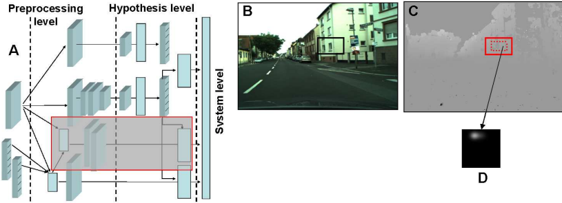
Fig. 7 Examples of stereo processing for elevation and distance calculation. A ) embedding into processing system B ) video image with object hypothesis C ) dense elevation map F^2(\mathbf{x}) , similar to distance map F^3(\mathbf{x}) . D ) population-coded elevation z^2(\mathbf{p}) resulting from this measurement. An analogous processing generates population coded-distance z^3(\mathbf{p}) . Such population codes may be more or less strongly multimodal, thus reflecting the uncertainty of the associated measurement.
