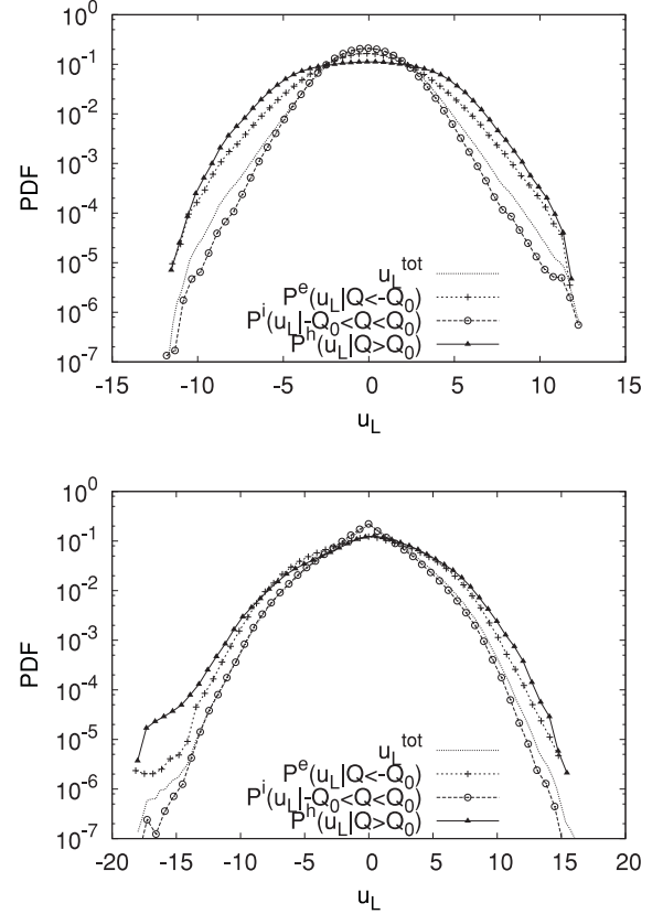
FIG. 6. Conditional pdf of Lagrangian velocity in the x direction with respect to the three-level Weiss field in the double periodic domain (top panel) and in the bounded circular domain (bottom panel). Note that u_L^{\text{tot}} refers to the unconditioned velocity.
