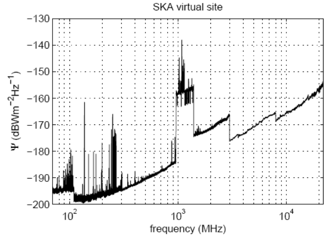
Fig. 2. SKA site measurements, median of spectra obtained during the 2005/2006 monitoring campaign in China, Argentina, South-Africa, and Australia.
