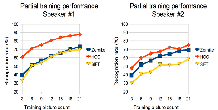
Fig. 5. Evolution curves of performance versus training database size
