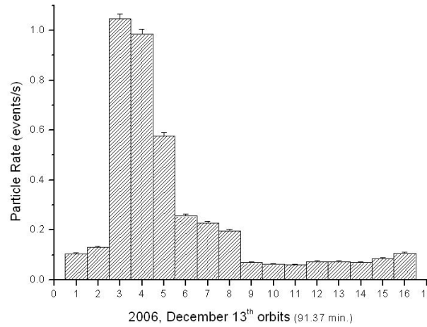
Figure 6: Light particles (Z<5) rate distribution during December the 13 th . The particle rate is calculated summing up the events recorded along each orbital revolution of the ISS. The climax of the solar event corresponds to the 3 rd -5 th orbit-time frame, i.e. from 03:03:16amUT to 07:38:09amUT.
