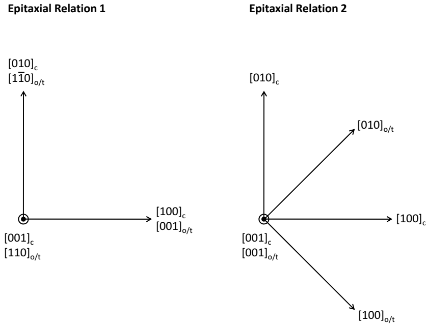
Figure 9. Sketch of the two epitaxial relations possible for the growth of orthorhombic (o) and tetragonal (t) SrRuO 3 films on SrTiO 3 (001) substrates. [001]_c is along the growth direction of the film.
