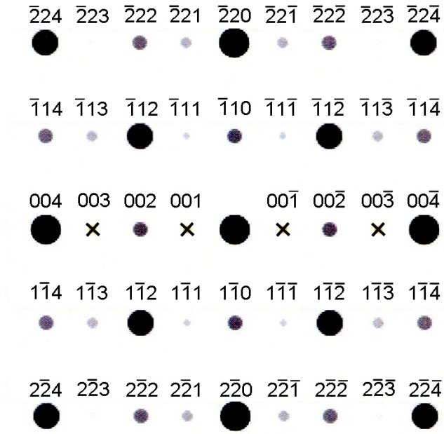
Figure 7. Simulated diffraction pattern for orthorhombic SrRuO_3 . Zone axis [110]_o , i.e. in a direction corresponding to equivalent zone axes in Figs. 5 and 6. Kinematically forbidden but dynamically appearing reflections are marked by crosses, among them the [001]_o reflection used during reconstruction of the dark-field images in those figures. Spot size is proportional to the intensity of the reflection. (Simulation performed by JEMS program [P. Stadelmann, EPFL Lausanne, Switzerland]).
