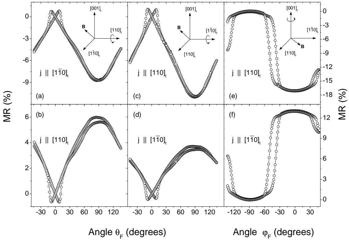
Figure 12. Sample SL3: T = 10 K, \mu_0 H = 8 T. Angular dependence of the magnetoresistance for magnetic field rotation in the (110)_t -, (\bar{1}10)_t - and (001)_t -planes. The current directions are indicated in each panel.
