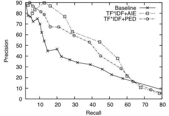
Figure 1: Recall/precision curves for topic tracking based on a combination of the tf-idf criterion and acoustic features.
