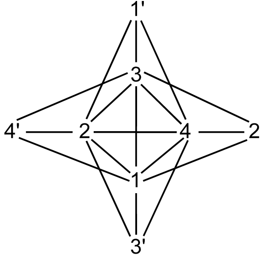
Figure 2.8: Graph G of Remark 2.70.
