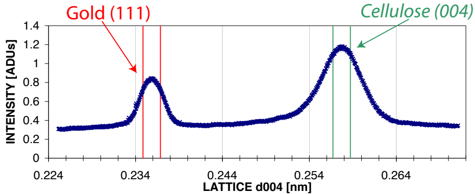
Fig. 3: Example of radial profile of cellulose (004) and gold (111) obtained from diffractogram integration
