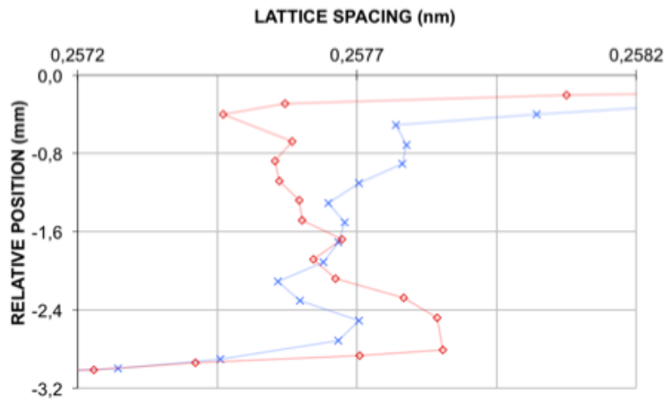
Fig. 4: Profiles of cellulose lattice spacing along the height of specimen 1, at the initial state ( \text{---}\times\text{---} ) and deformed state ( \text{---}\diamond\text{---} ). The macroscopic strain applied is \varepsilon^- = -0.194\% and \varepsilon^+ = 0.184\% .
