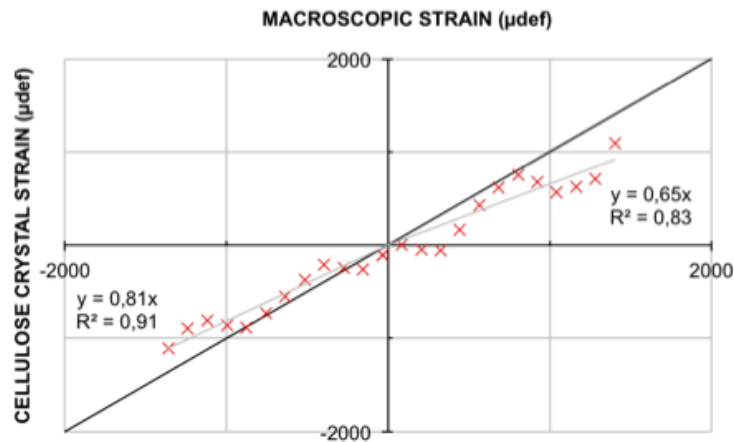
Fig 6: Relationship between cellulose crystal strain and wood macroscopic strain (specimen 1). × experimental results, — linear regression of experimental results, — 1:1 line
