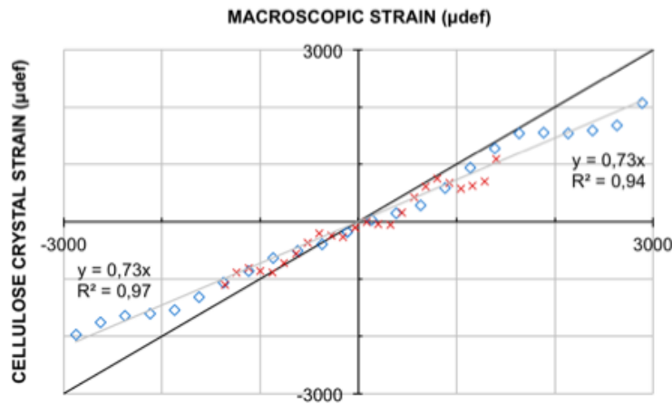
Fig. 8: Relationship between cellulose crystal strain and wood macroscopic strain (specimen 1) at two levels of applied strain; firstly at \Delta\varepsilon = 0.1903\% (×) and secondly increased at \Delta\varepsilon = 0.3957\% (◇). The grey lines (—) indicates linear regressions on data relative to the larger strain level.
