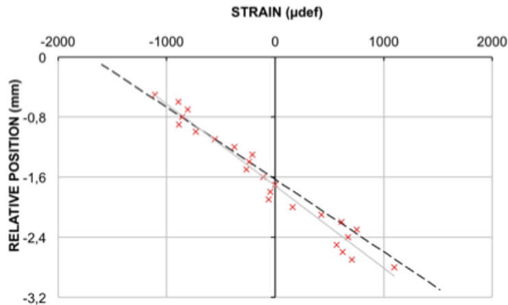
Fig. 5: Profile of cellulose crystal strain ( \times ) and wood macroscopic strain ( \text{---} ) along the height of specimen 1. The gray line ( \text{---} ) indicates linear regression of the cellulose crystal strain.
