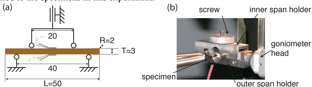
Fig. 1: (a) Schematic view of the four-point bending device and specimen dimensions (all dimensions in mm). \epsilon^- and \epsilon^+ is the strains measured with a strain gage on the upper (compressive) and lower (tensile) side, respectively. (b) Photography of four-point bending device specially designed for the X-ray goniometer head.
