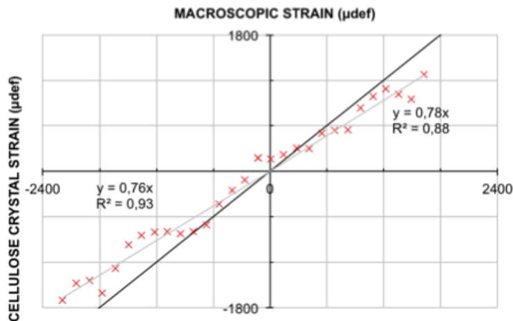
Fig 7: Relationship between cellulose crystal strain and wood macroscopic strain (specimen 2) × experimental results, — regression line of experimental results, — 1:1 line
