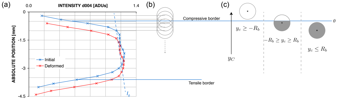
Fig. S1: (a) Profiles of signal intensity along specimen height y , at initial and deformed states. (b) beam overlap for successive shoots (c) relationship between beam centre position and diffracting wood area.
