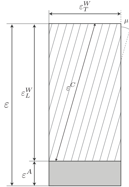
Figure 9: Schematic representation of the sources of longitudinal deformation in wood. Total strain \varepsilon can be divided into a contribution from the cell-wall \varepsilon^W , that depend on the crystal strain \varepsilon^C through the MFA \mu , and an additive contribution \varepsilon^A that does not involve the deformation of crystalline material.
