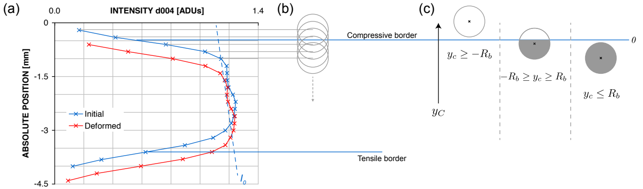
Fig. S1: (a) Profiles of signal intensity along specimen height y , at initial and deformed states. (b) beam overlap for successive shoots (c) relationship between beam centre position and diffracting wood area.
