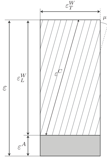
Figure 9: Schematic representation of the sources of longitudinal deformation in wood. Total strain \varepsilon can be divided into a contribution from the cell-wall \varepsilon_L^W , that depend on the crystal strain \varepsilon^C through the MFA \mu , and an additive contribution \varepsilon^A that does not involve the deformation of crystalline material.
