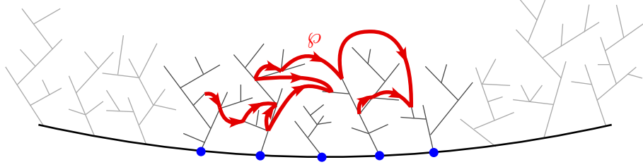
Figure 5: The set overflowed by the path \varphi is the set of (blue) large dots. Note that the middle tree is overflowed although it is not visited. The arrows on the arcs of \varphi point from corners to their successors in the Bouttier–Di Francesco–Guitter bijection.
