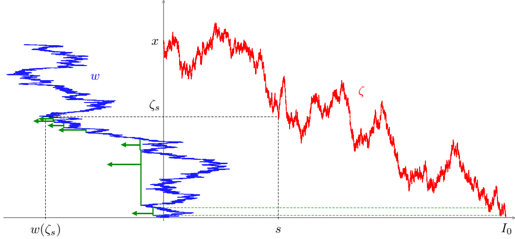
Figure 10: Visual aid for the proof of Lemma 12. On this picture, the timescale of \zeta and W is horizontal, whereas the timescale of w is vertical. The point s satisfies \zeta_s = \zeta_{\infty} = \inf\{t : w(t) = w(\zeta_s)\} . We represented by (green) solid lines the seven longest excursions of w - \underline{w} before time \zeta_s , and the (green) arrows represent the minimum of \widehat{W} on the intervals that correspond in the timescale of W to these excursions.
