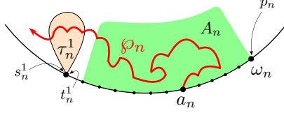
Figure 7: The path \varphi_n passing through the tree \tau_n^1 .
