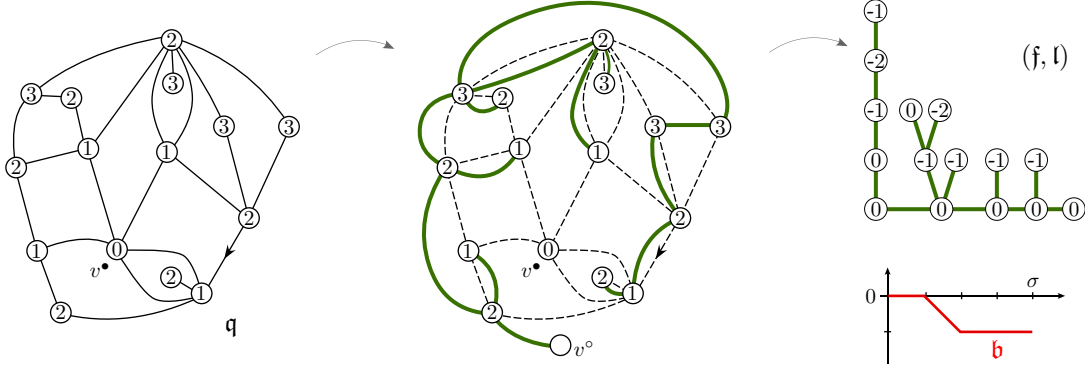
Figure 3: The mapping from \mathcal{Q}_{n,\sigma}^* onto \mathfrak{F}_\sigma^n \times \mathcal{B}_\sigma . In this picture, n = 10 and \sigma = 4 .
