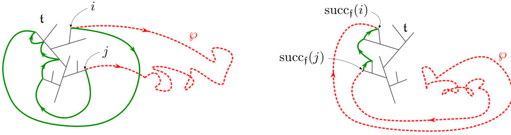
Figure 9: On this picture, t is the only part of f represented. The dashed (red) line represents the path \varphi (in q_f ) and the (green) solid path is the path in q_t . Both first cases are represented.
