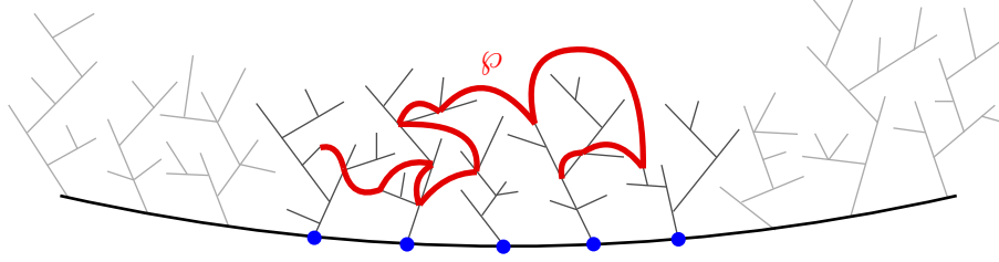
Figure 5: The set overflowed by the path \varphi is the set of (blue) large dots.
