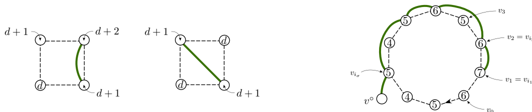
Figure 2: Left. Adding the new edge to an internal face. Right. Example of the operation on the external face. In this example, \mathbf{b} = (0, -1, -1, -2, -2, -1) .
