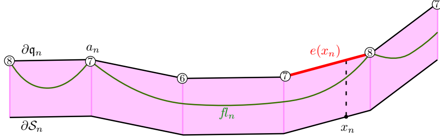
Figure 8: Approaching a point x_n \in \partial\mathcal{S}_n with a point a_n \in f_n .
