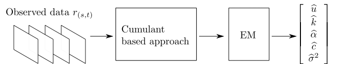
Fig. 1. Flowchart of the proposed noise identification method.
