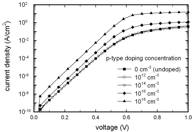
FIG. 5. Simulated j - V curves with various doping concentrations in pentacene. This result points out that the assumption of zero doping is applicable as long as the dopant density lies below the injected carrier density at the anode.
