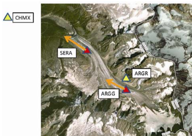
Figure 2. Local view of the Argentière glacier with locations of dedicated GPS stations. The average flow velocities of the two glacier stations ARGG and SERA are indicated schematically, evaluated to 13.3 cm/day (in this work) and 16.8 cm/day [3].
