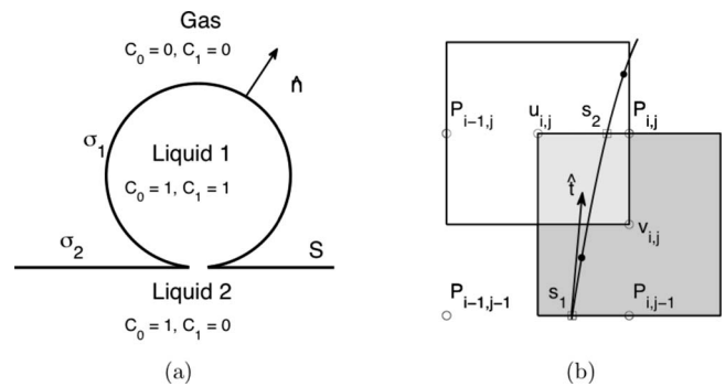
FIG. 3. (a) Initial configuration of a drop of liquid 1 at rest on a reservoir of liquid 2. Simulations are initiated at the onset of coalescence, with a thin neck joining the drop and reservoir. Initial values of the concentration functions C_0 and C_1 are shown. (b) Staggered grid used, shown around the point where v_{i,j} is defined. The black curve is the interface, interpolated between markers (black dots).
