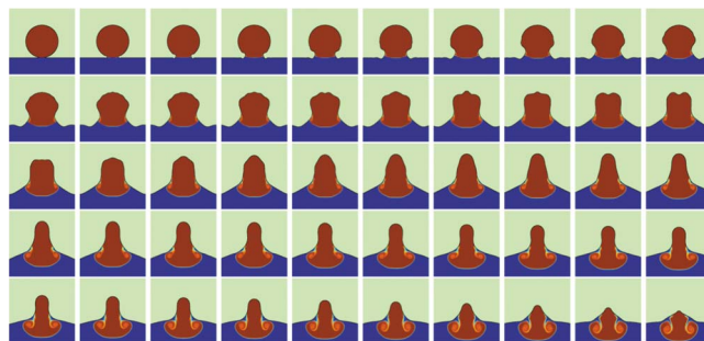
FIG. 6. (Color online) Simulation of the coalescence of a drop of larger surface tension than that of the reservoir, R_\sigma=\sigma_2/\sigma_1=0.92 . Each image shown is 0.04 nondimensional time units apart. Despite the low Ohnesorge number, Oh=0.001 , the surface tension variations prevent partial coalescence.
