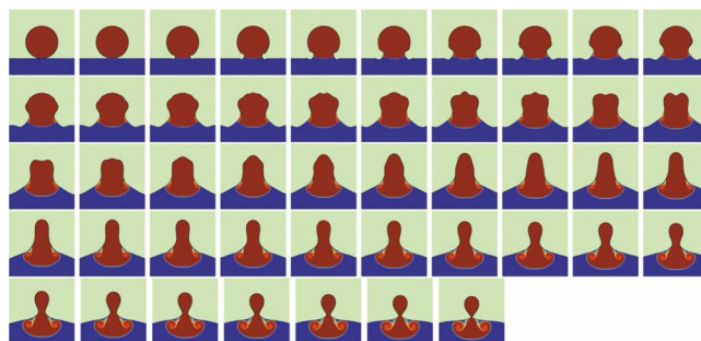
FIG. 7. (Color online) Simulation of the coalescence of a drop with slightly larger surface tension than the reservoir, R_\sigma=\sigma_2/\sigma_1=0.9667 . Each image shown is 0.04 nondimensional time units apart and Oh=0.001 . Partial coalescence is observed, although the drop is smaller than it would be in the absence of the surface tension mismatch.
