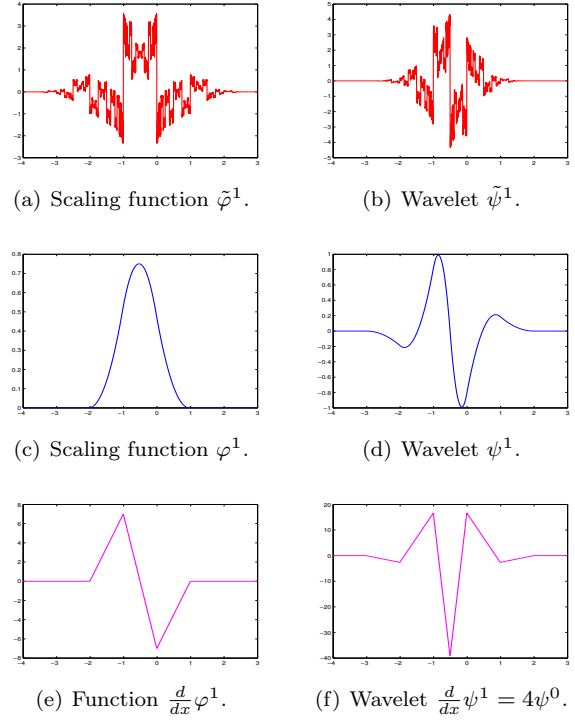
Fig. 4: Example of biorthogonal generators and primal derivatives: case of B-Spline generators (\varphi^1, \tilde{\varphi}^1) with 3 vanishing moments.
