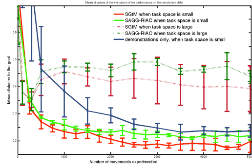
Figure 5: Evaluation of the performance of the robot under the learning algorithms: SAGG-RIAC and SGIM-D, when the task space is small or 20 times larger. We plotted the mean distance to the benchmark points over several runs of the experiment.
