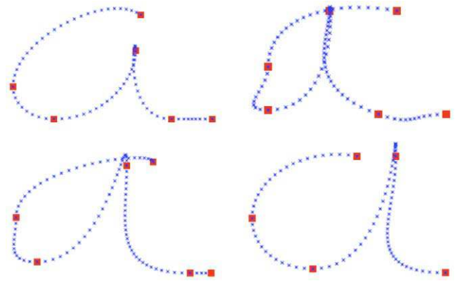
Figure 16. Within-writer inter-trial variability produced by the BAP model trajectory generation. Four trajectories obtained by computing P(\ddot{\theta}_1^{0:T} \ddot{\theta}_2^{0:T} | [L=a][W = \text{Estelle}][\lambda_p = 1]) . doi:10.1371/journal.pone.0020387.g016
