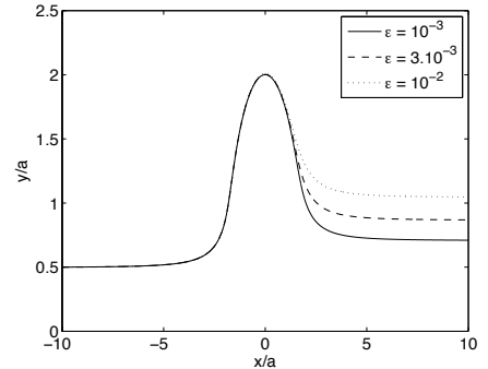
FIG. 5: Trajectory from the point x/a=-10 , y/a=0.5 , z/a=0 for different values of the roughness \epsilon a
