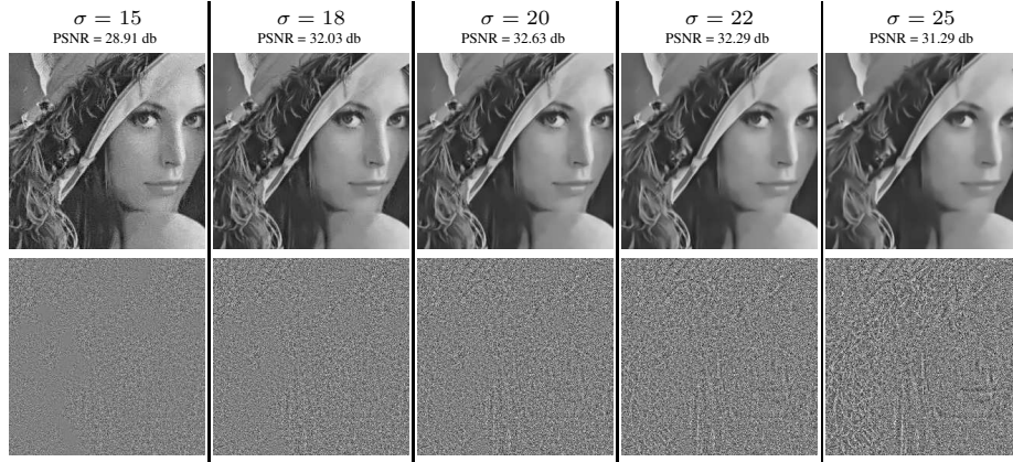
Fig. 2. Denoising with the plugin Adaptive NL-means filter ANL_{\sigma, n} \tilde{\mathbf{u}}_{ANL} of the artificially corrupted Lena image (WGN, \sigma = 20 ) with different estimations of the noise variance and experiments with the “method noise” (bottom).
