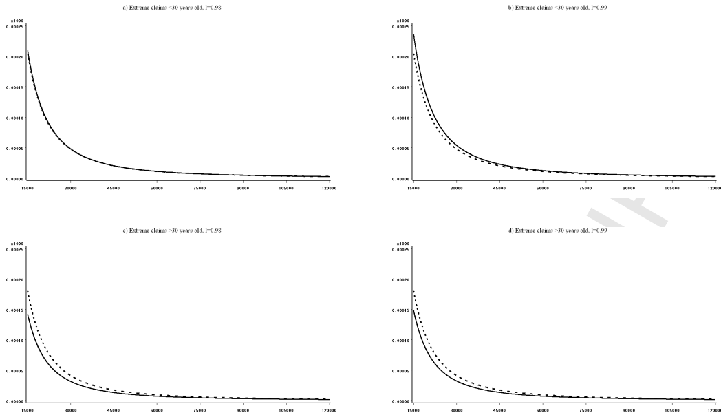
Fig. 1. KIBMCE with l = 0.99 and l = 0.98 (solid line) and KMCE (dashed line) estimators of automobile claims from an insurance company. In a) and b) younger policyholders and in c) and d) older policyholders.
