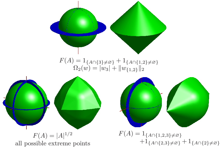
Figure 5.5: Unit balls for structured sparsity-inducing norms, with the corresponding submodular functions and the associated norm, for \ell_2 -relaxations. For each example, we plot on the left side the sets K_A defined in §5.4 as well as the convex hulls of their unions in green (on the right side).
