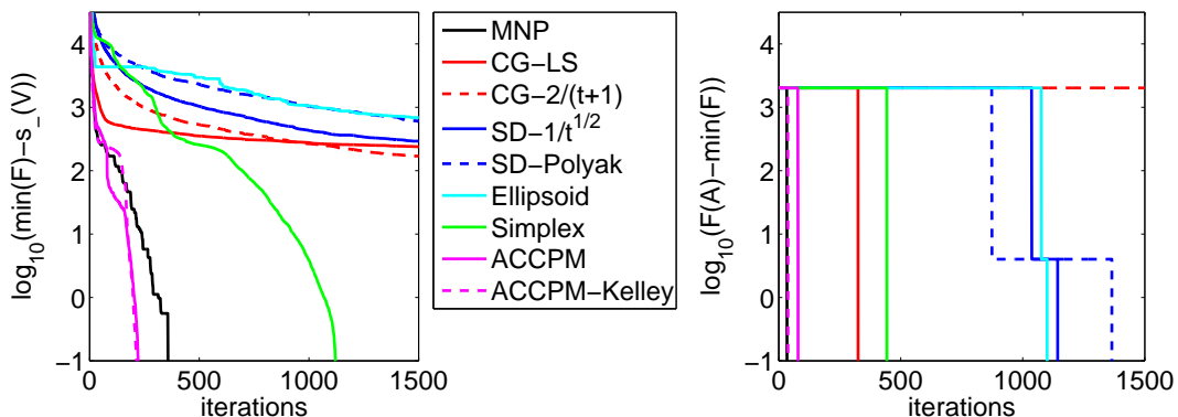
Figure 12.2: Submodular function minimization results for “Genrmf-wide” example: (left) optimal value minus dual function values in log-scale vs. number of iteration. (Right) Primal function values minus optimal value in log-scale vs. number of iterations. Best seen in color.
