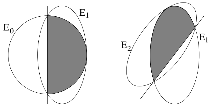
Figure 7.1: Two iterations of the ellipsoid method, showing how the intersection of a half-plane and an ellipsoid may be inscribed in another ellipsoid, which happens to have a smaller volume.
