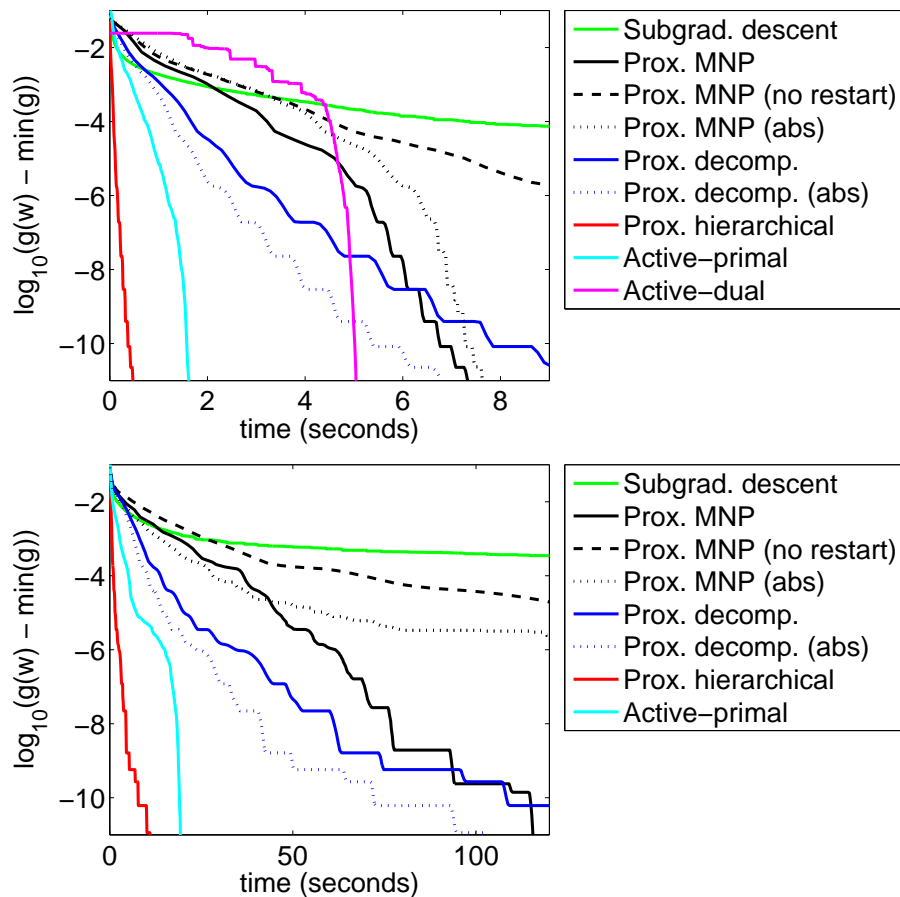
Figure 12.11: Running times for convex optimization for a regularized problem: several methods are compared; top: small-scale problems ( p = 127 ), bottom: medium-scale problem p = 511 ). See text for details. Best seen in color.
