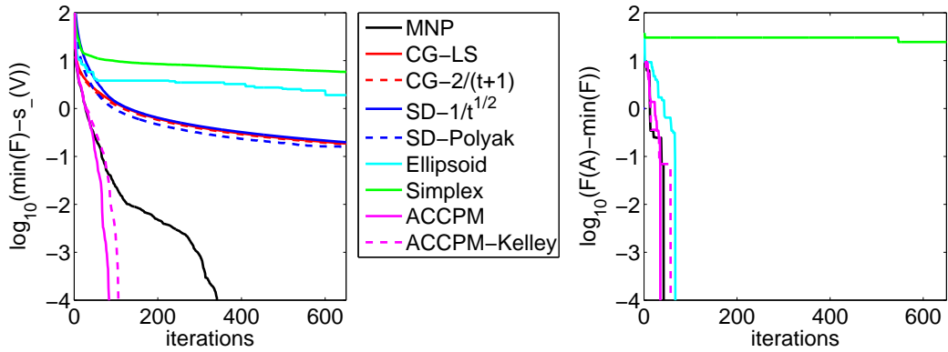
Figure 12.4: Submodular function minimization results for “Two-moons” example: (left) optimal value minus dual function values in log-scale vs. number of iteration. (Right) Primal function values minus optimal value in log-scale vs. number of iterations. Best seen in color.
