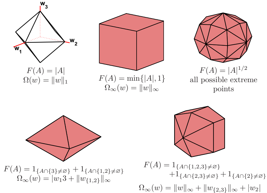
Figure 5.3: Unit balls for structured sparsity-inducing norms, with the corresponding submodular functions and the associated norm.
