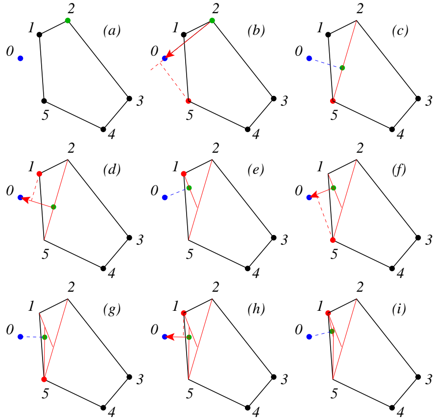
Figure 9.2: Illustration of Frank-Wolfe conditional gradient algorithm: starting from the initialization (a), in steps (b),(d),(f),(h), an extreme point on the polytope is found in steps (c),(e),(g),(i), a line search is performed. Note the oscillations to converge to the optimal point (especially compared to Figure 9.1).
