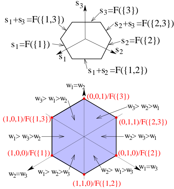
Figure 4.1: (Top) representation of B(F) for F(A) = 1_{|A| \in \{1,2\}} and p = 3 (projected onto the set s(V) = F(V) ). (Bottom) associated dual polytope, which is the 1-sublevel set of f (projected on the hyperplane w^\top 1_V = 0 ).
